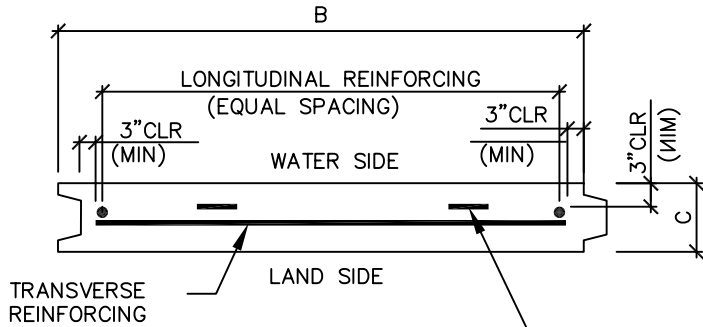
TOP OF SLAB VIEW
