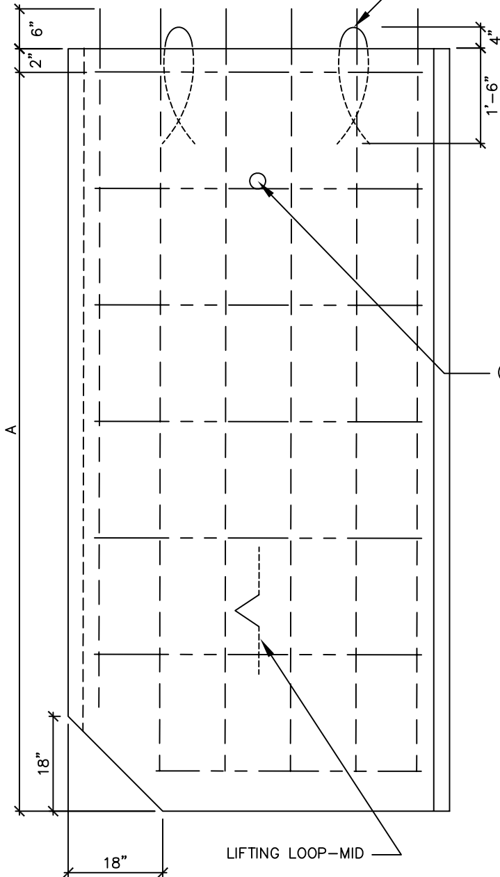
TOP OF SLAB VIEW
